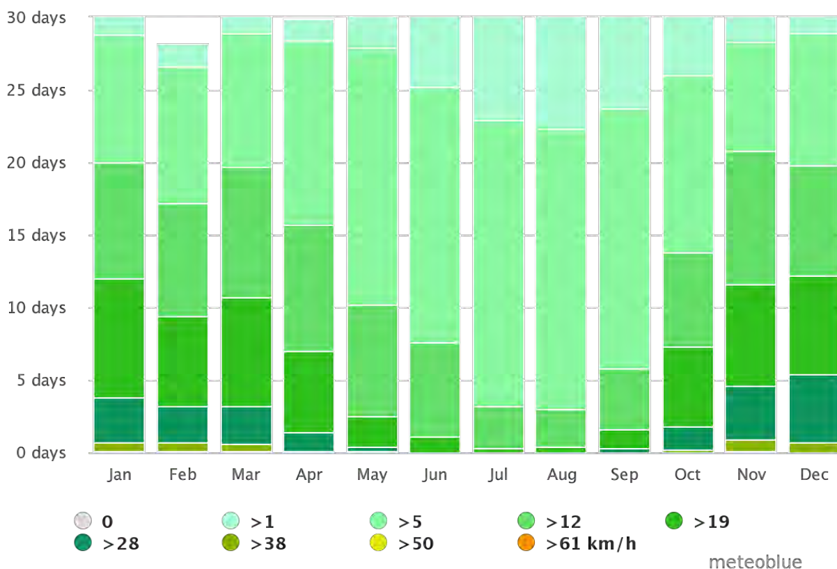
Figure 10. Windspeeds by month experienced for Coombs (meteoblue).
