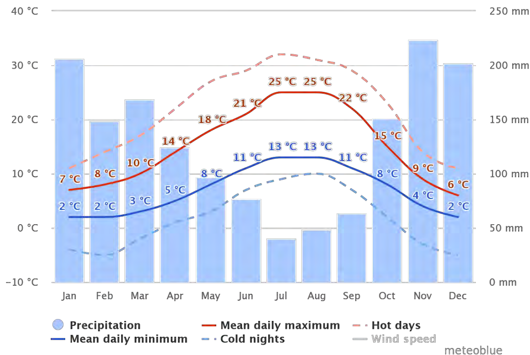
Figure 8. 30-year modelled climate averages for Coombs (meteoblue).
