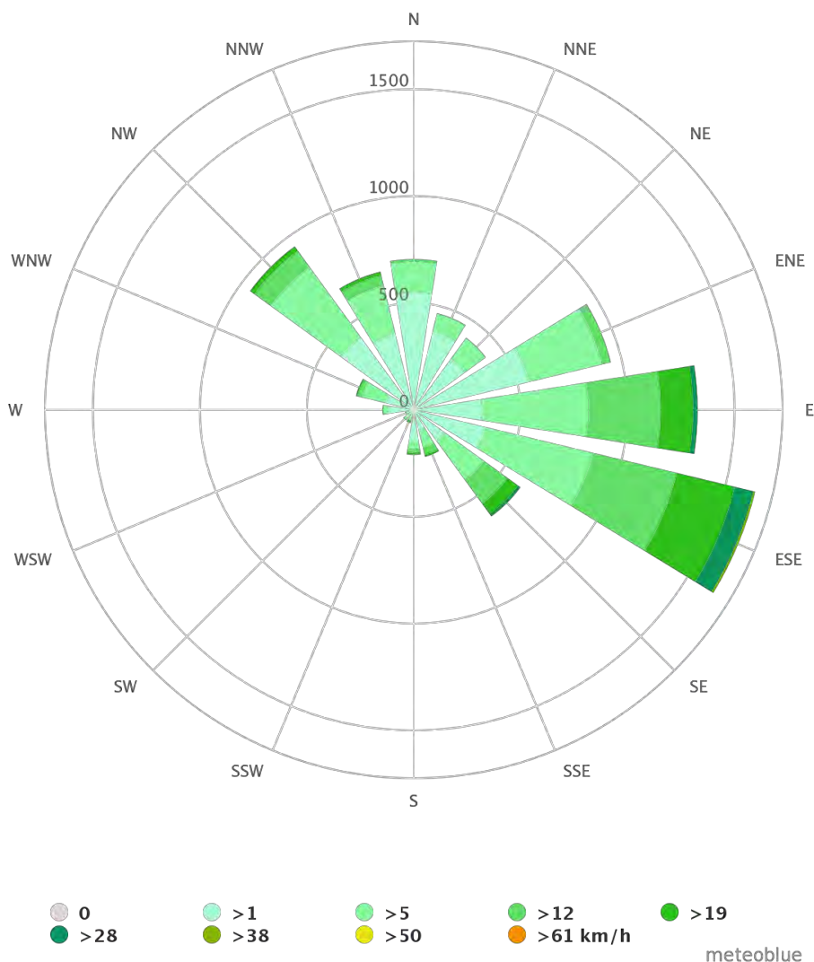
Figure 9. Wind rose diagram for Coombs (meteoblue). The diagram shows cumulative hours (the wind rose radius) at an average windspeed from each cardinal direction during the average year (1990-2020).
