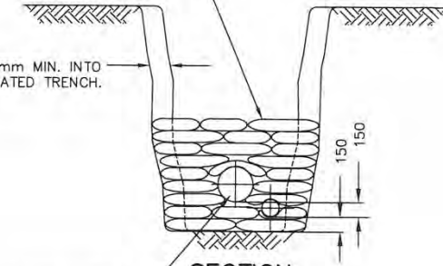
SANITARY SEWER SECTION
