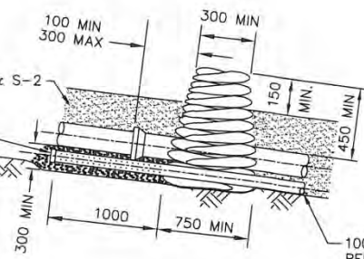
SANITARY SEWER SECTION
