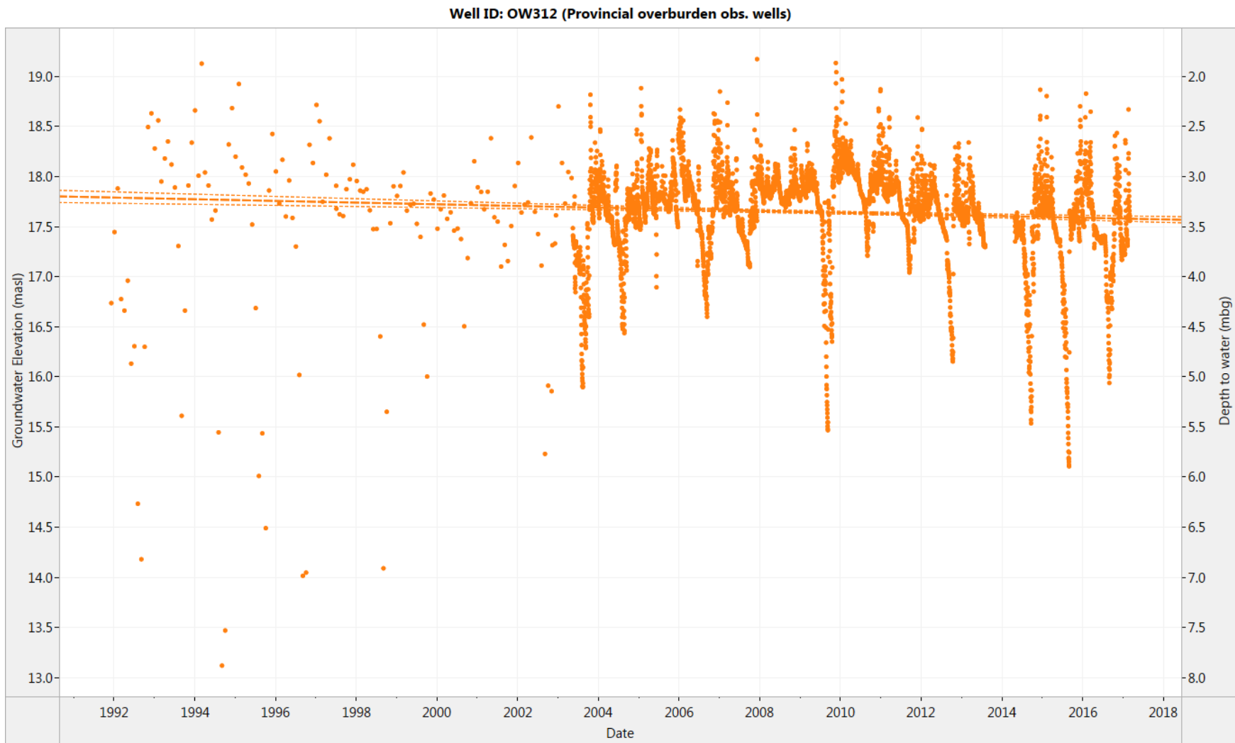
Figure 3. OW312: Historical daily water level (1991-2016) and trend line estimation (2003-2016)
