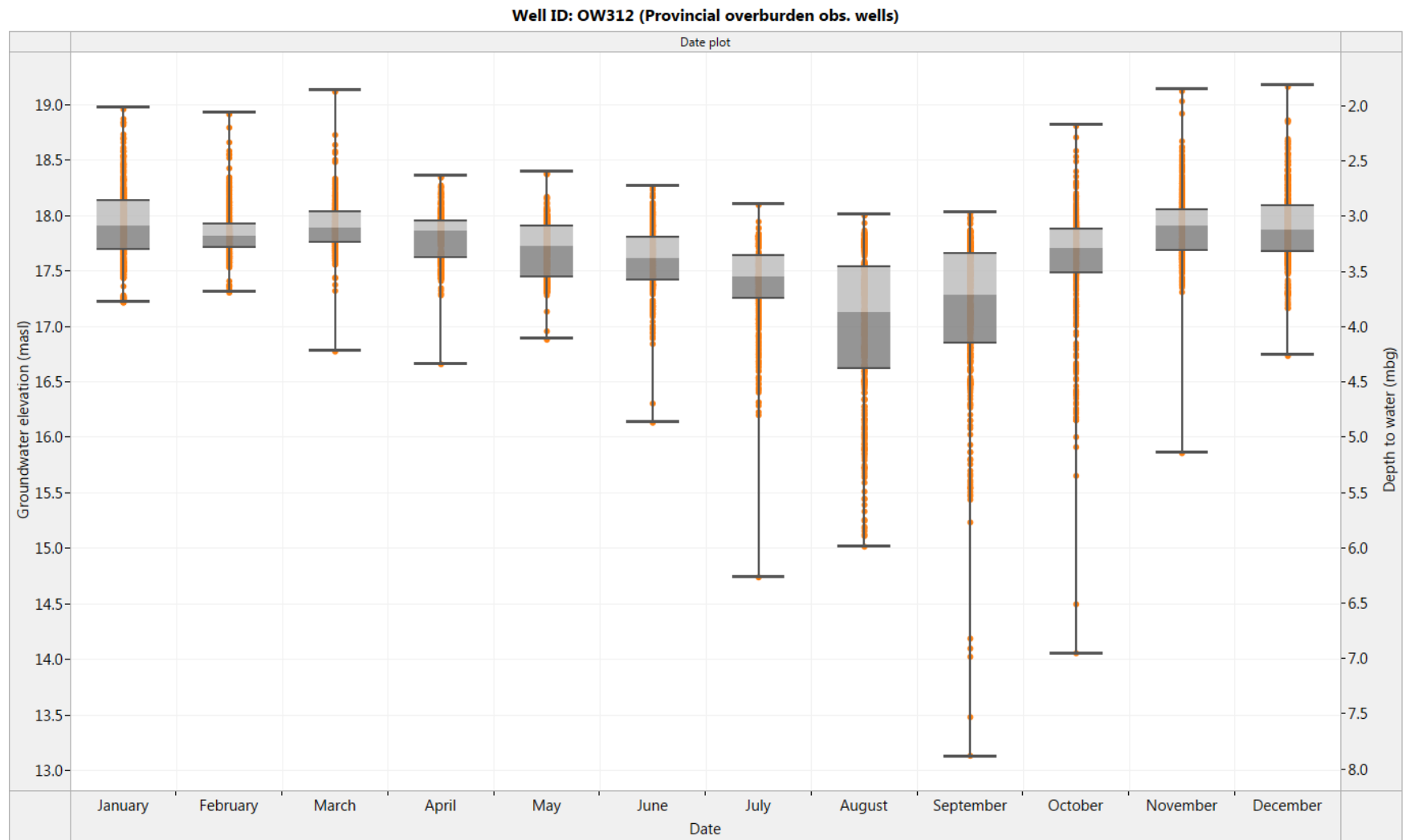
Figure 6. OW312: Box and Whisker diagram for historical monthly groundwater level fluctuation (1991-2016)
