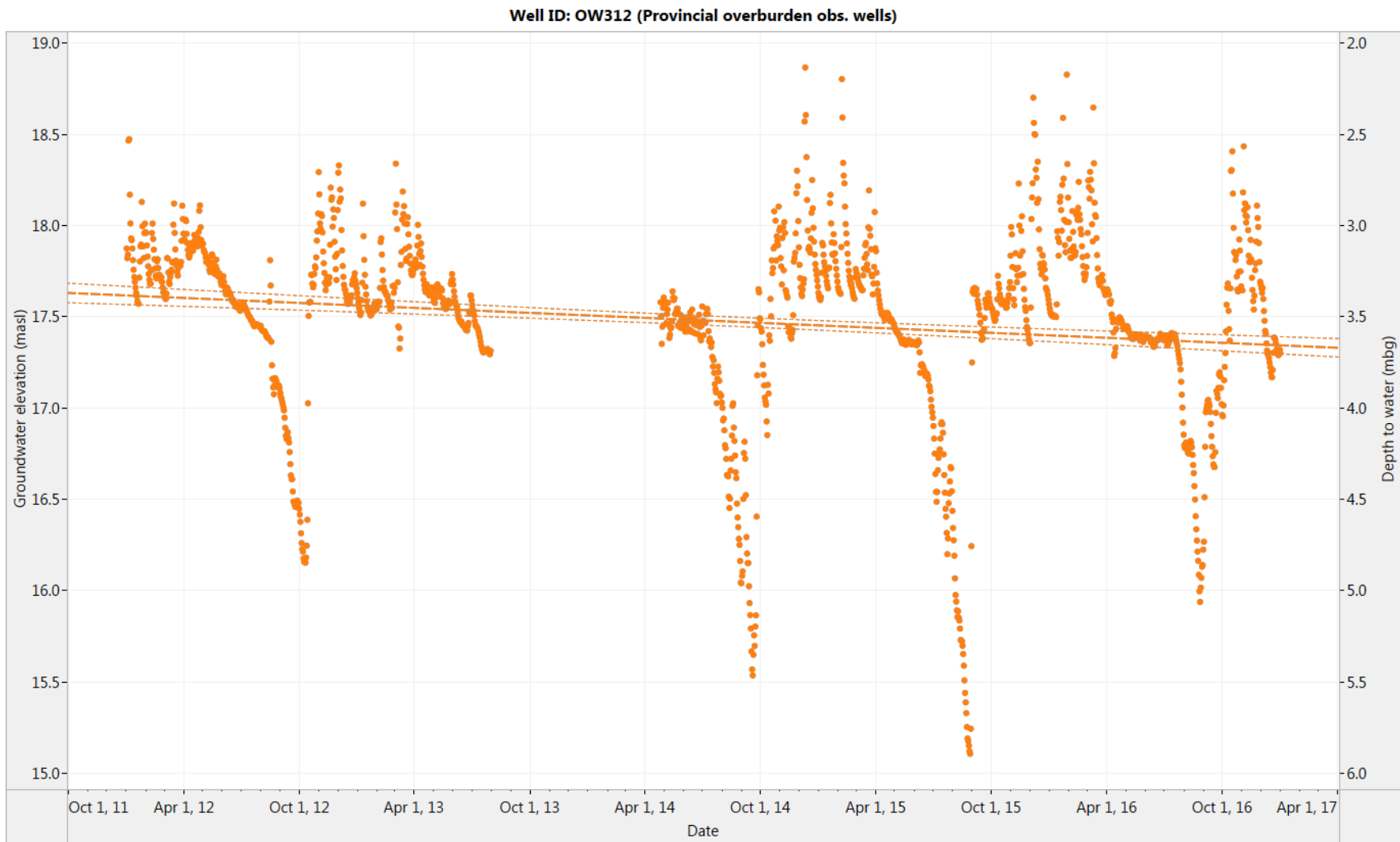
Figure 4. OW312: Water level and trend line estimation for the last five years (2012-2016)
