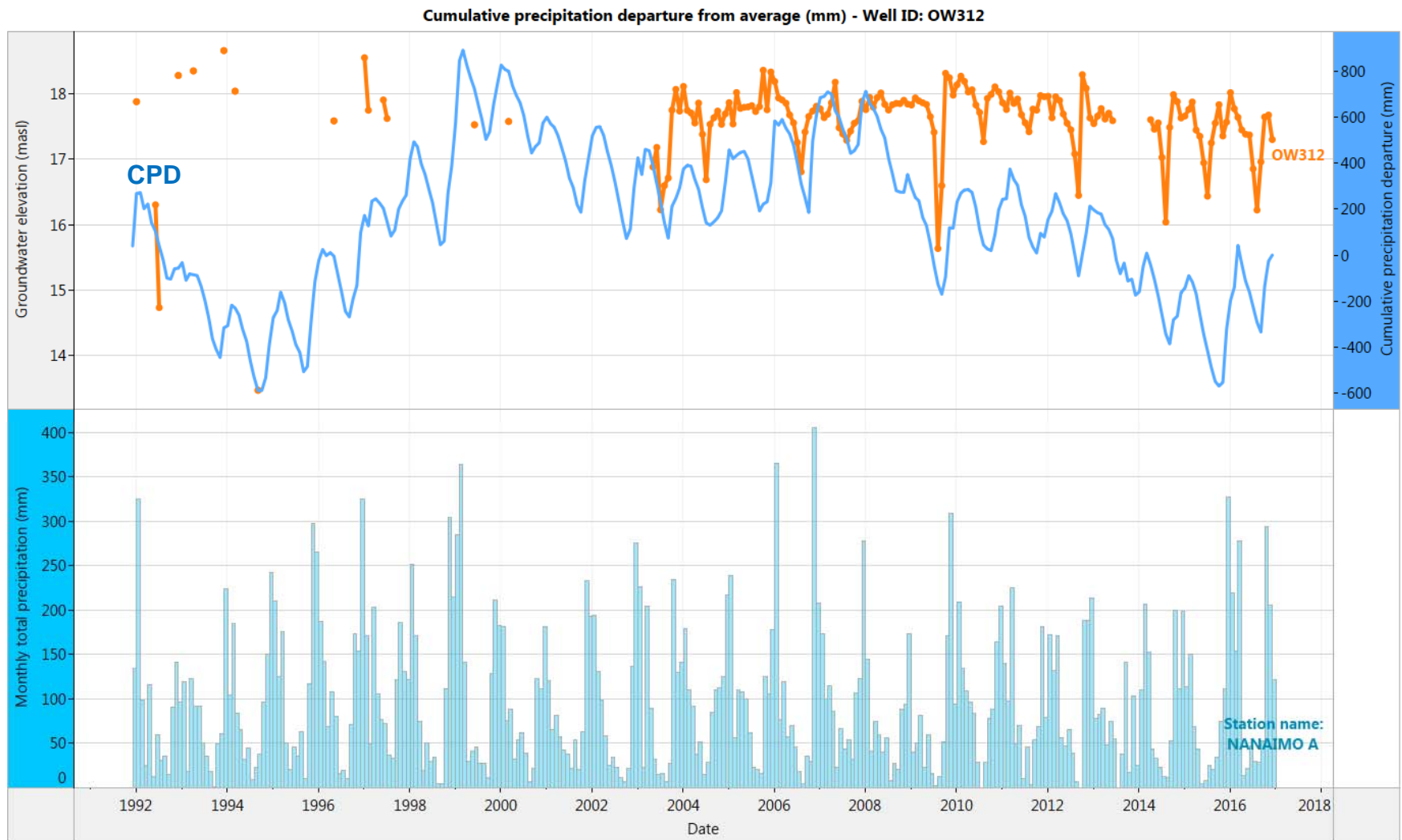
Figure 8. OW312: Month end groundwater levels compared to cumulative precipitation departure curve and total monthly precipitation (1991-2016)
