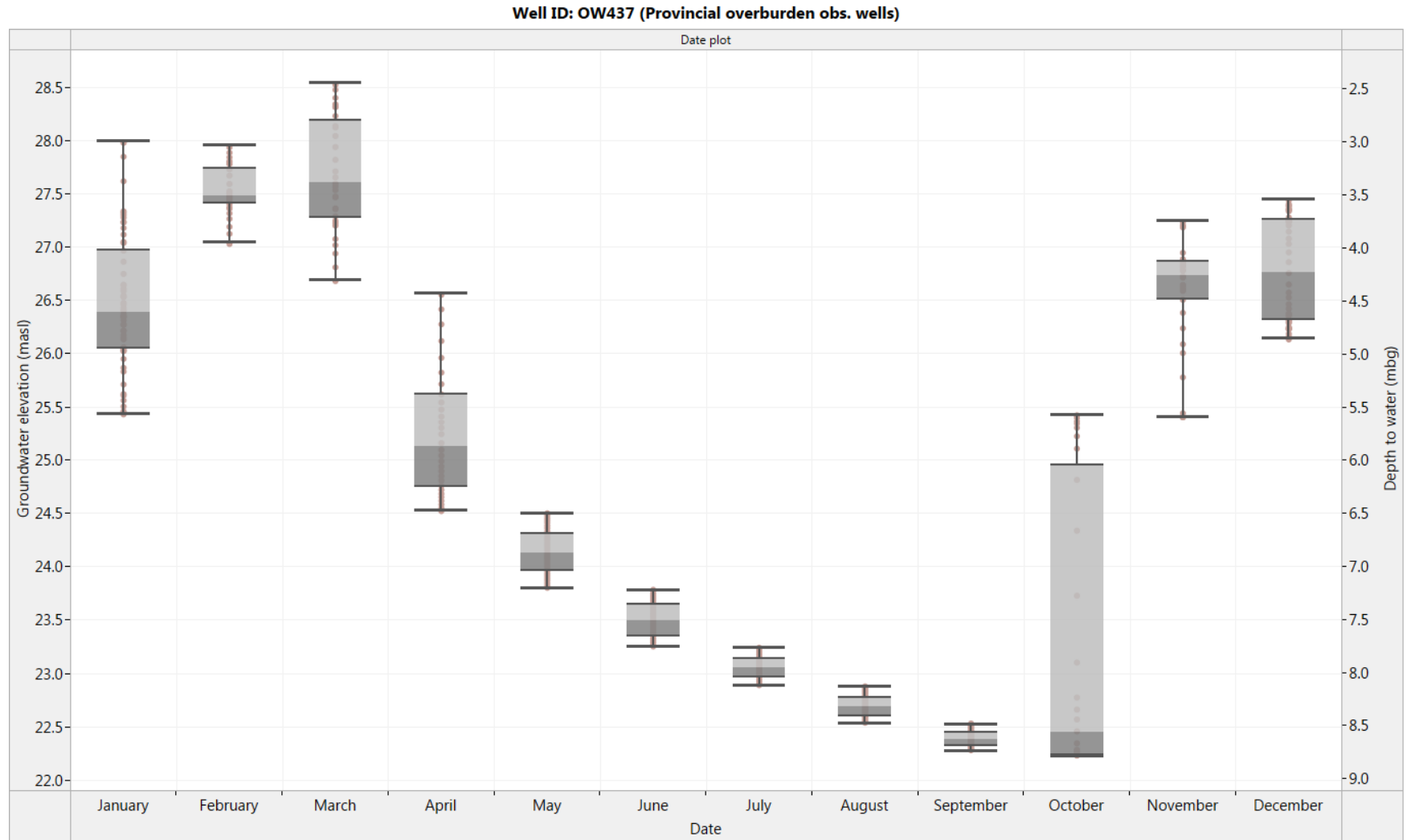
Figure 7. OW437: Box and Whisker diagram for historical monthly groundwater level fluctuation (2015-2016)
