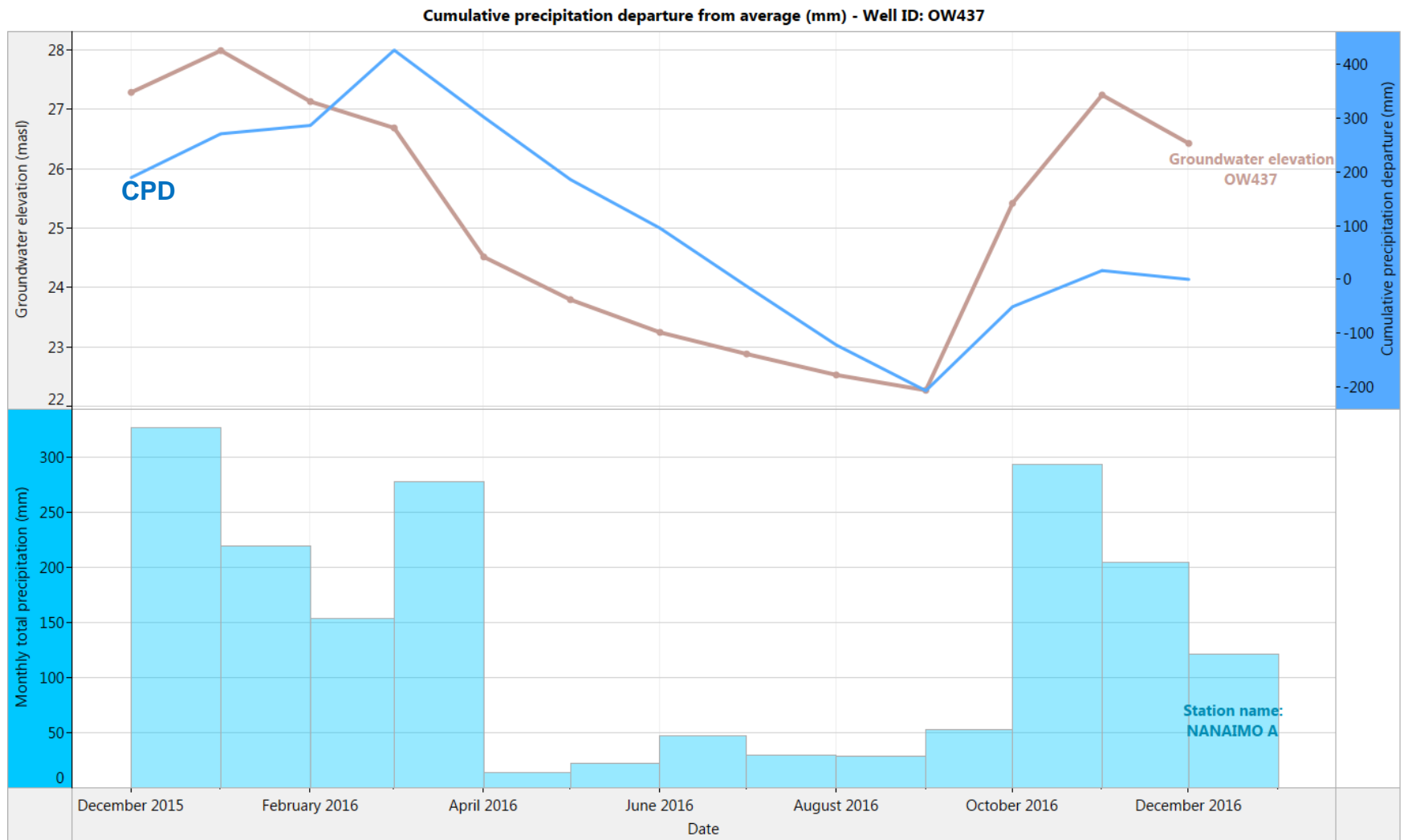
Figure 9. OW437: Month end groundwater levels compared to cumulative precipitation departure curve and total monthly precipitation (2015-2016)
