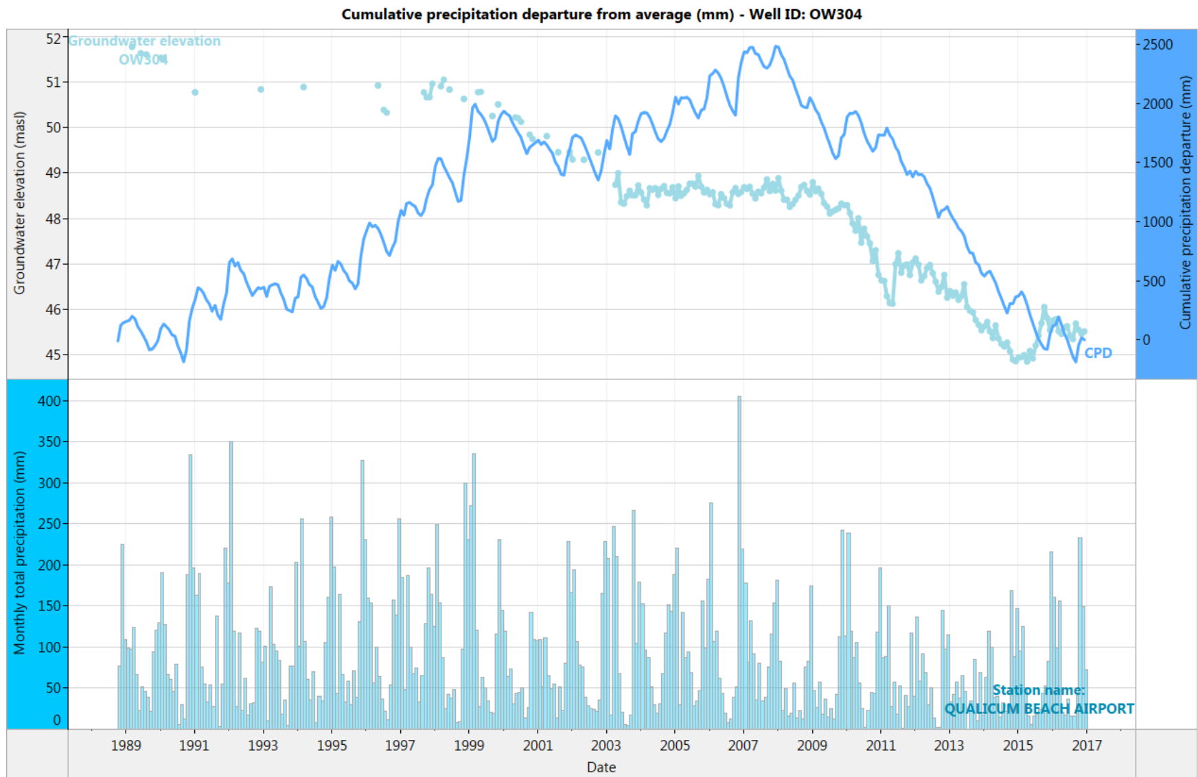
Figure 18. OW304: Month end groundwater levels compared to cumulative precipitation departure curve and total monthly precipitation (1988-2016)
