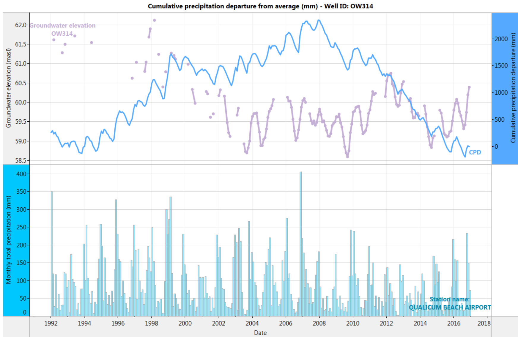
Figure 19. OW314: Month end groundwater levels compared to cumulative precipitation departure curve and total monthly precipitation (1992-2016)
