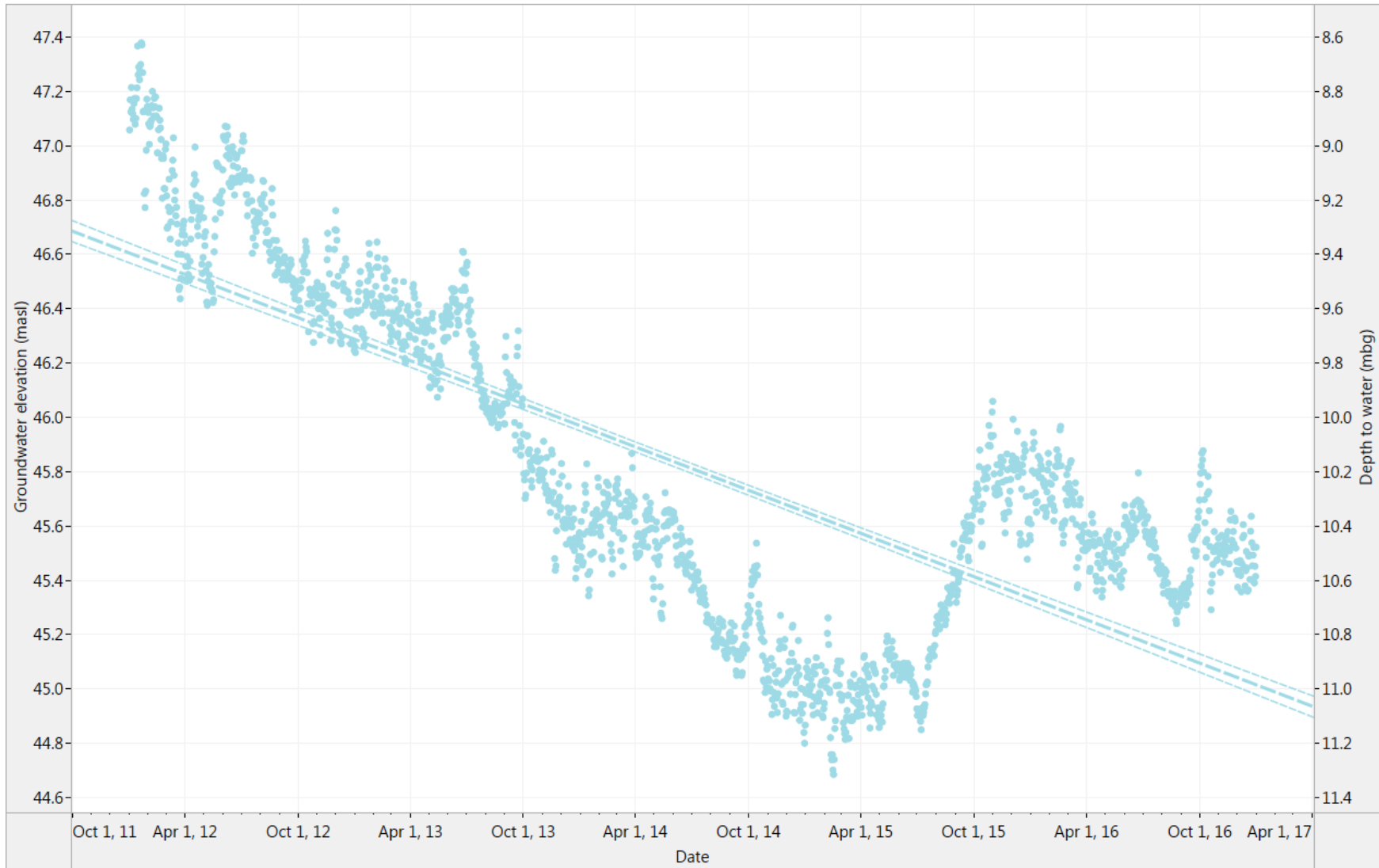
Figure 7. OW304: Water level and trend line estimation for the last five years (2012-2016)
