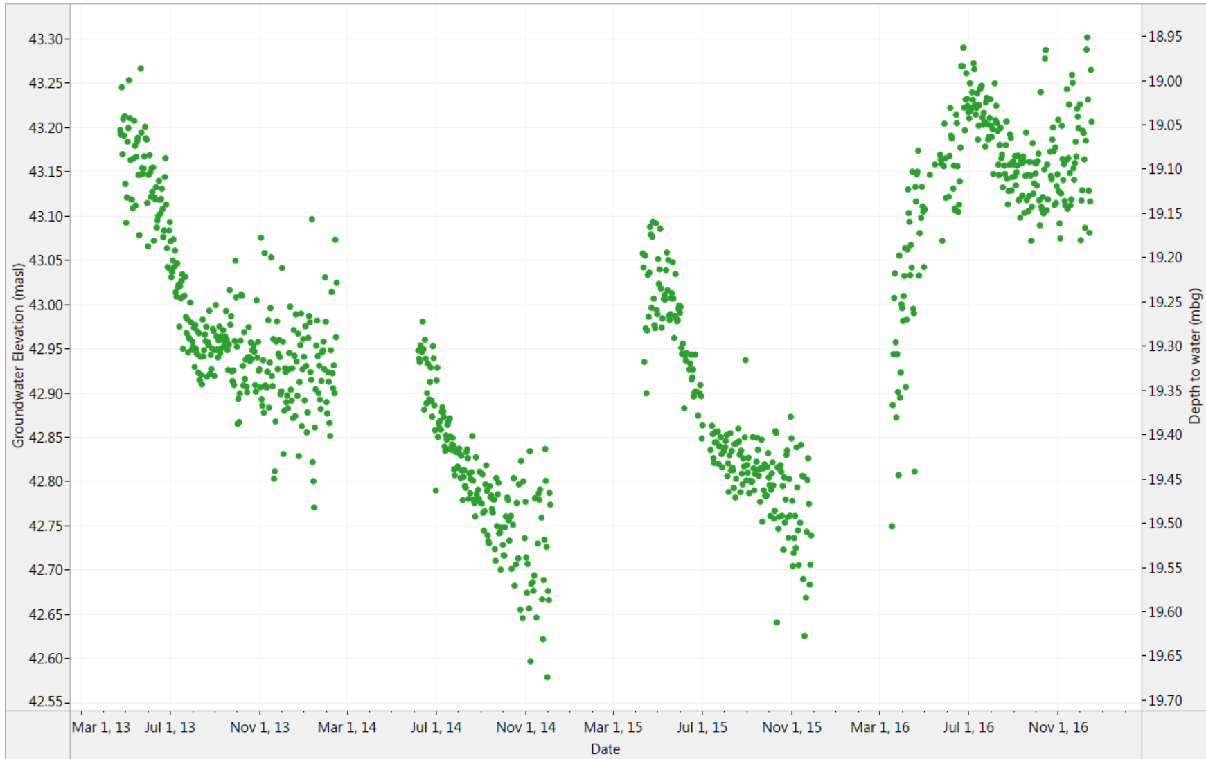
Figure 4. Fourneau: Historical water level (2013-2016)
