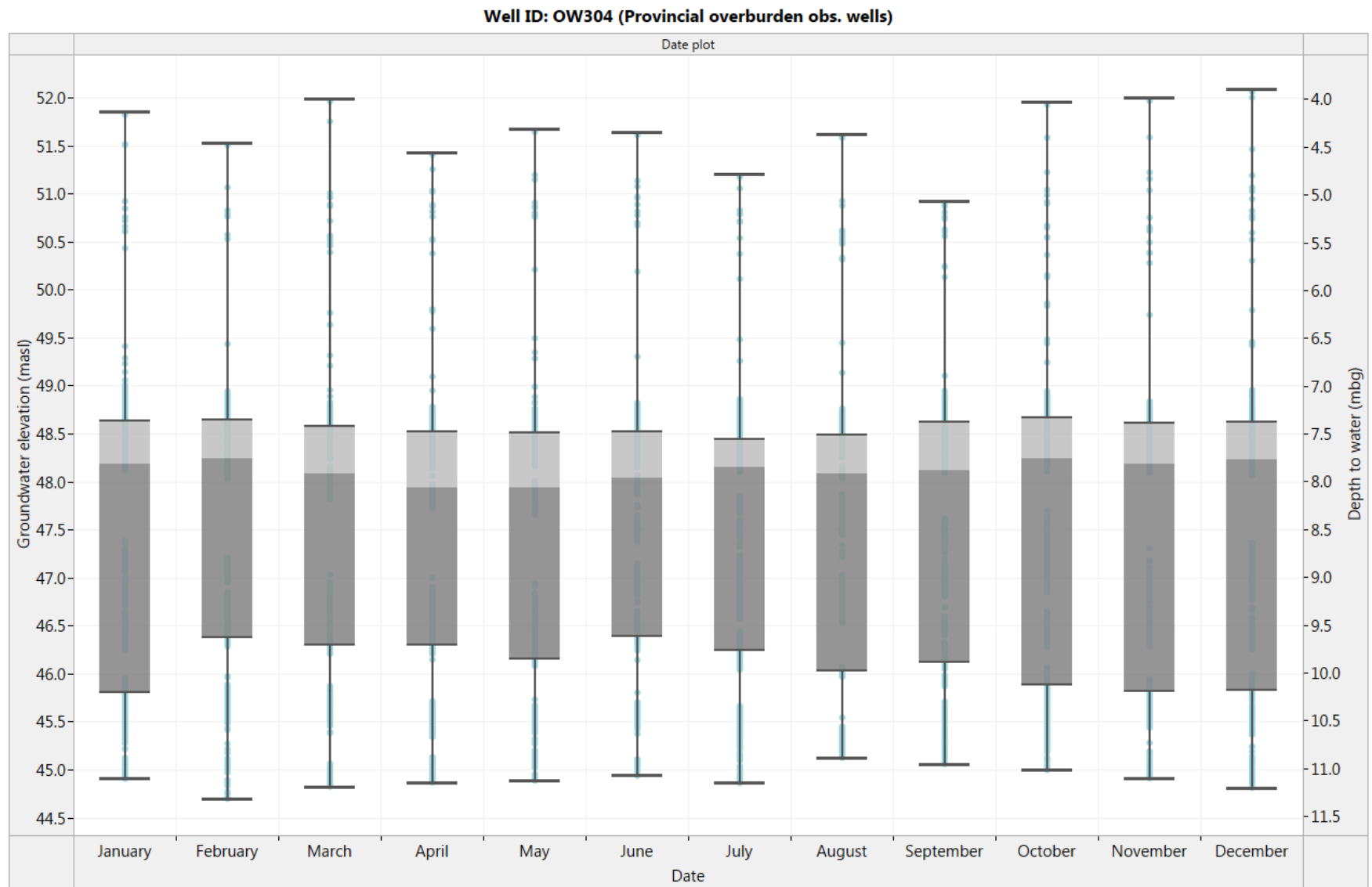
Figure 13. OW304: Box and Whisker diagram for historical monthly groundwater level fluctuation (1988-2016)
