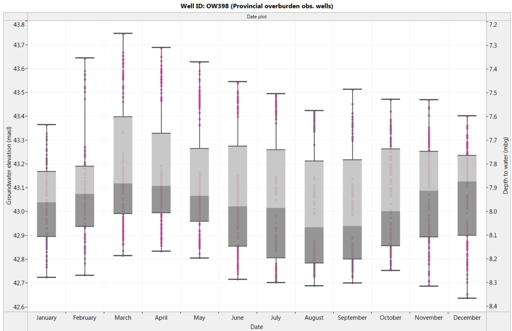
Figure 12. OW398: Box and Whisker diagram for historical monthly groundwater level fluctuation (2013-2016)
