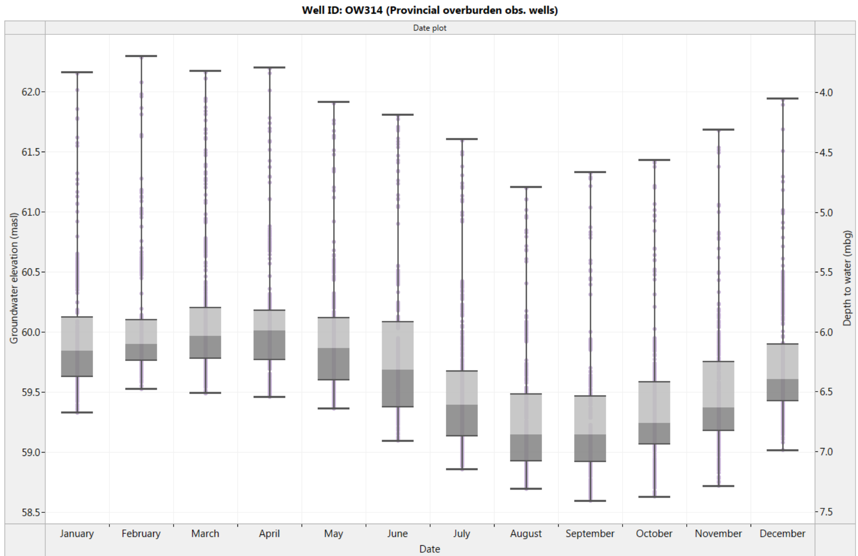
Figure 14. OW314: Box and Whisker diagram for historical monthly groundwater level fluctuation (1992-2016)
