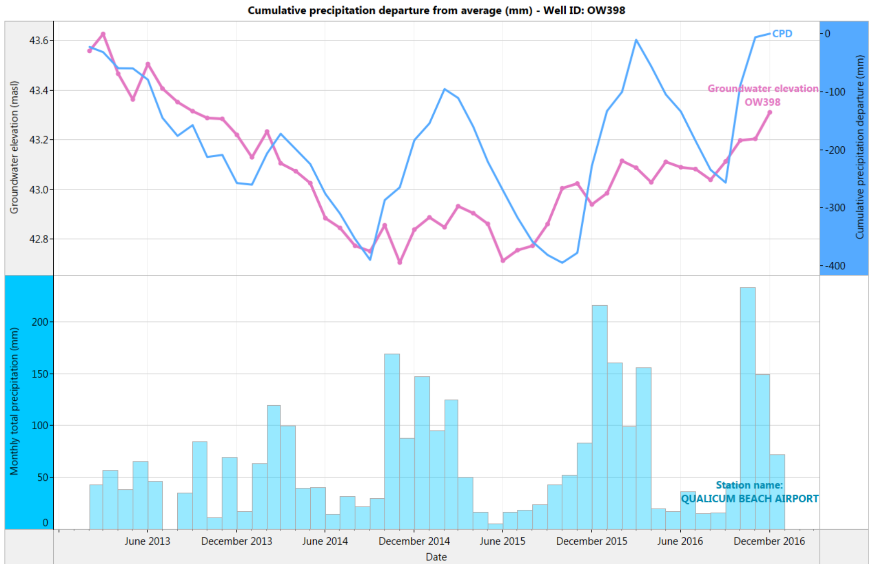
Figure 17. OW398: Month end groundwater levels compared to cumulative precipitation departure curve and total monthly precipitation (2013-2016)
