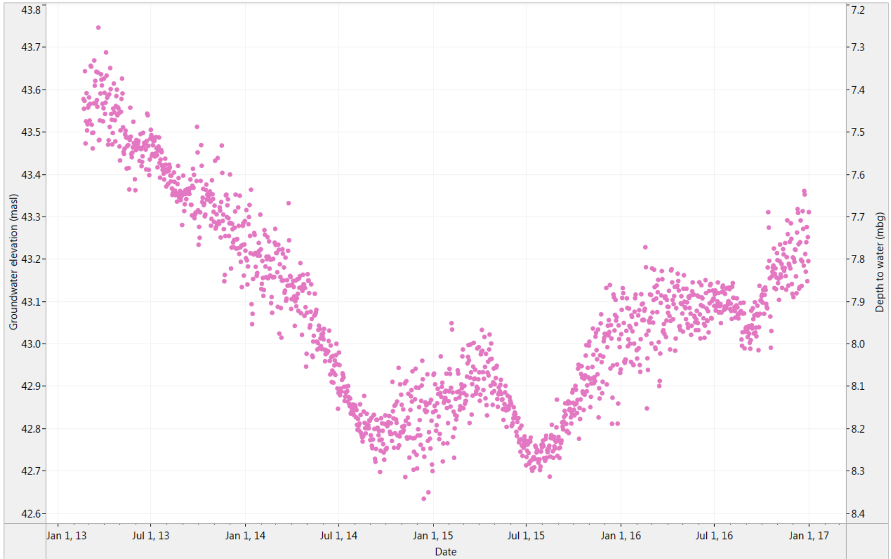
Figure 5. OW398: Historical water level (2013-2016)
