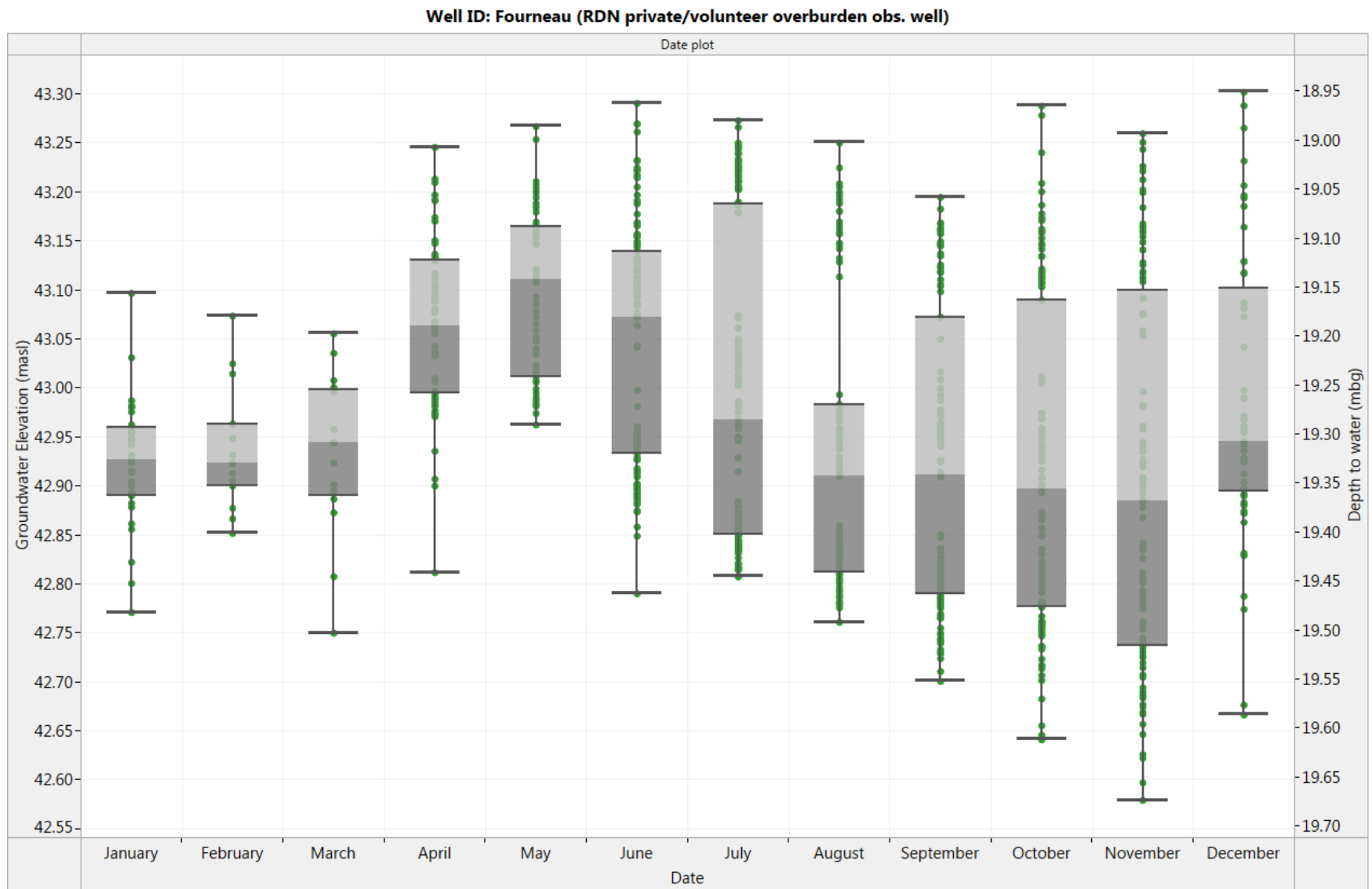
Figure 11. Fourneau: Box and Whisker diagram for historical monthly groundwater level fluctuation (2013-2016)
