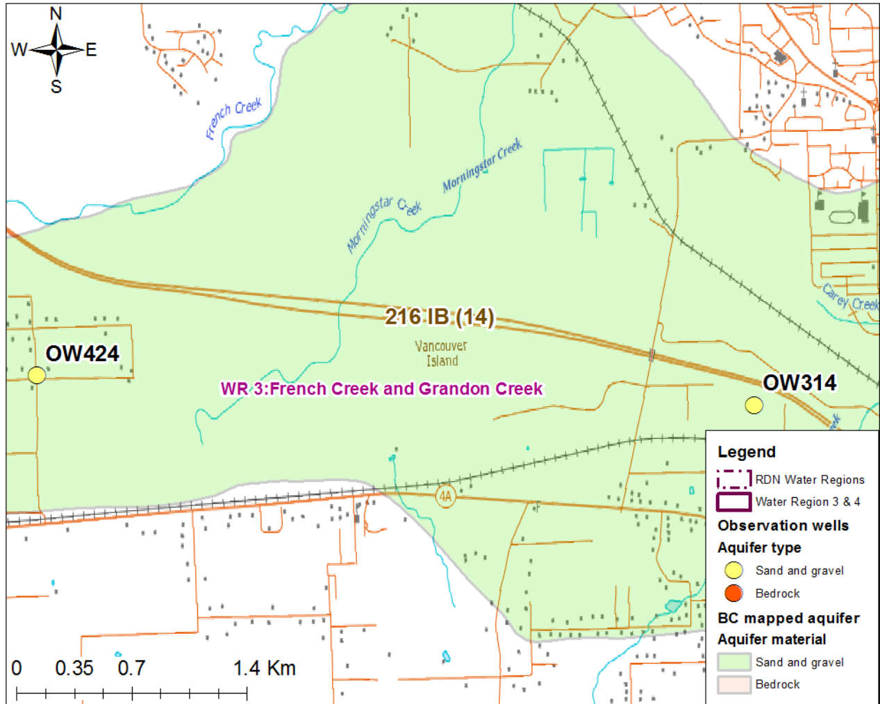
Figure 3. Location of observation wells OW314 and OW424
