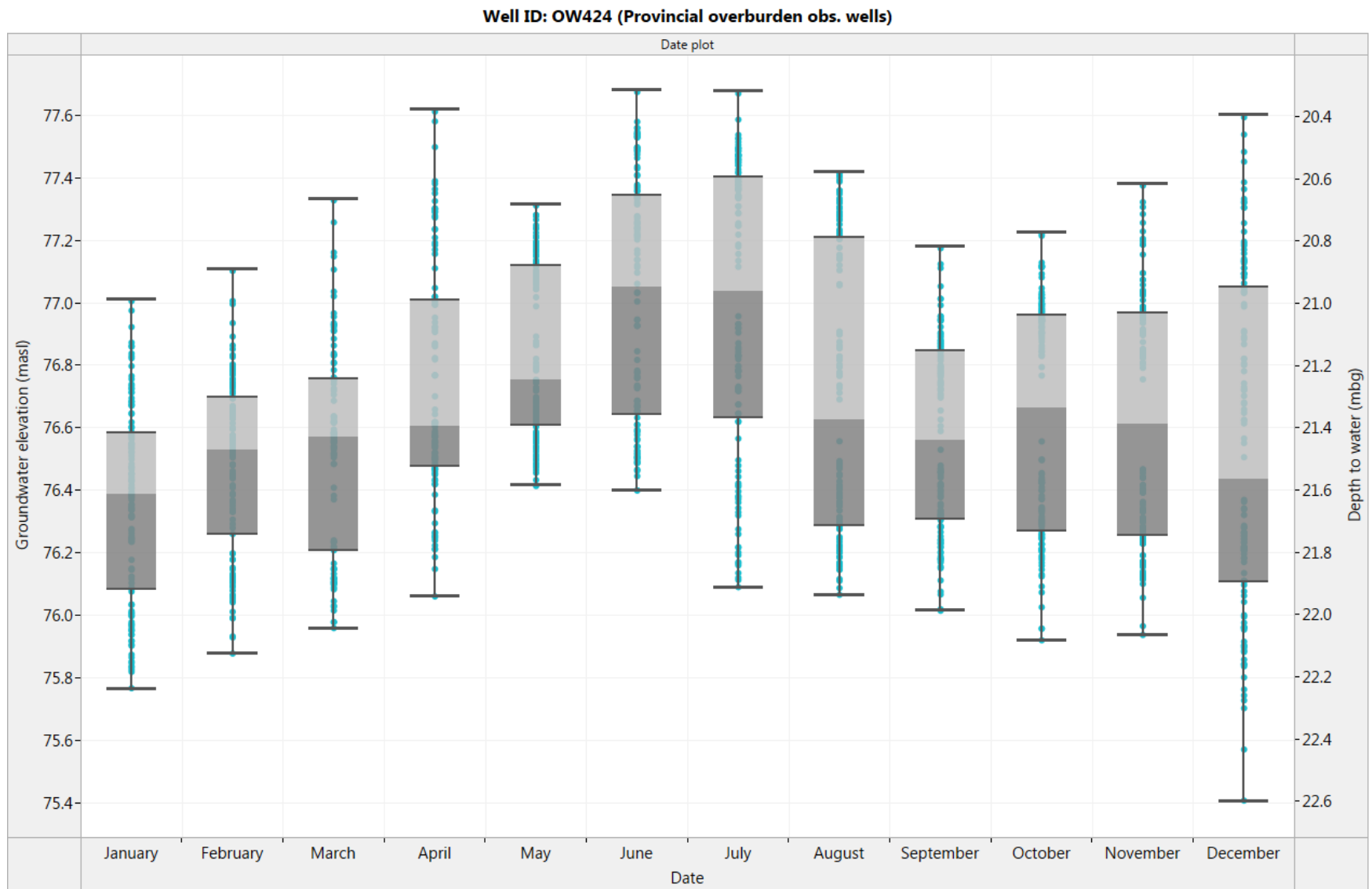
Figure 15. OW424: Box and Whisker diagram for historical monthly groundwater level fluctuation (2013-2016)
