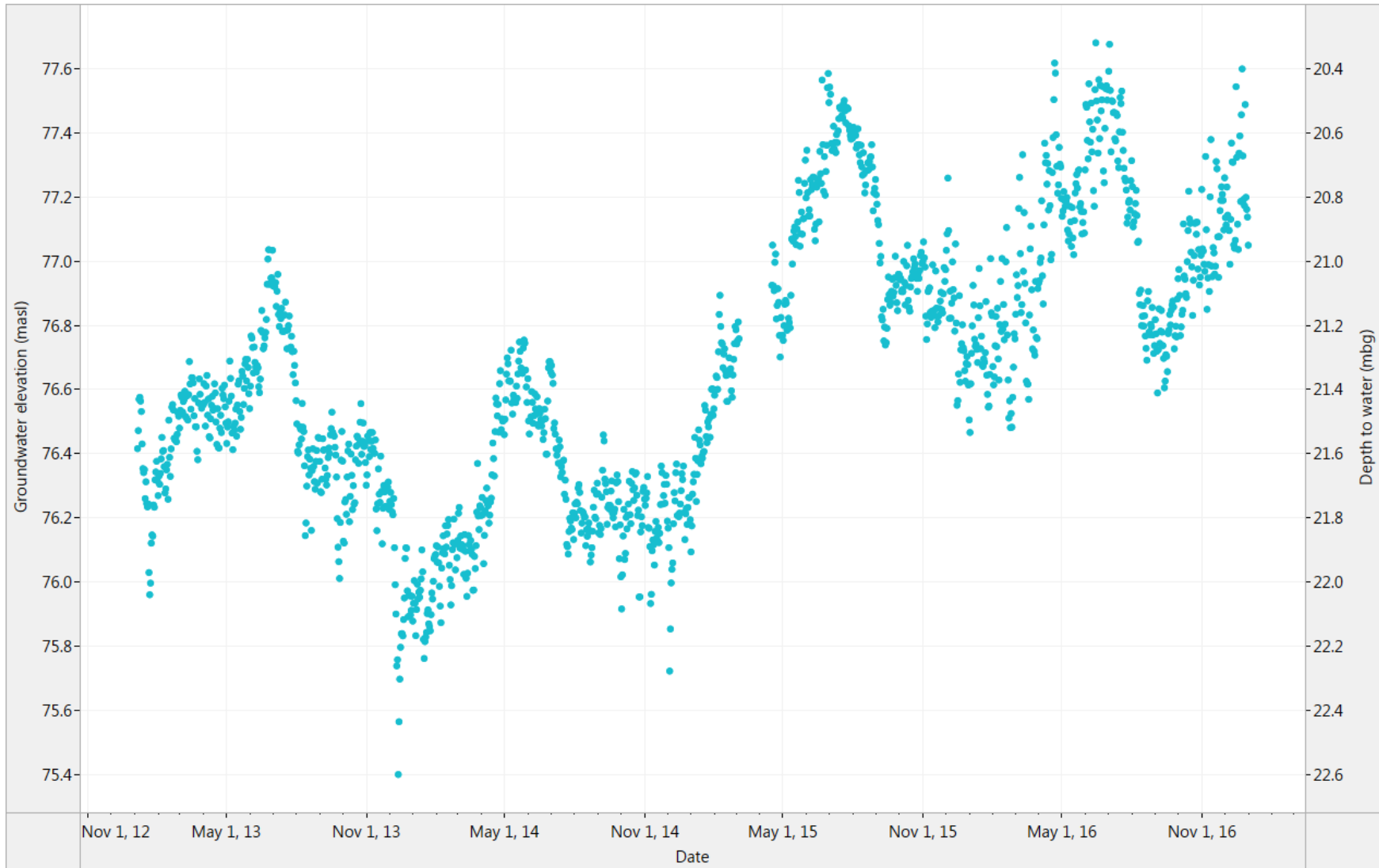
Figure 10. OW424: Historical water level (2013-2016)
