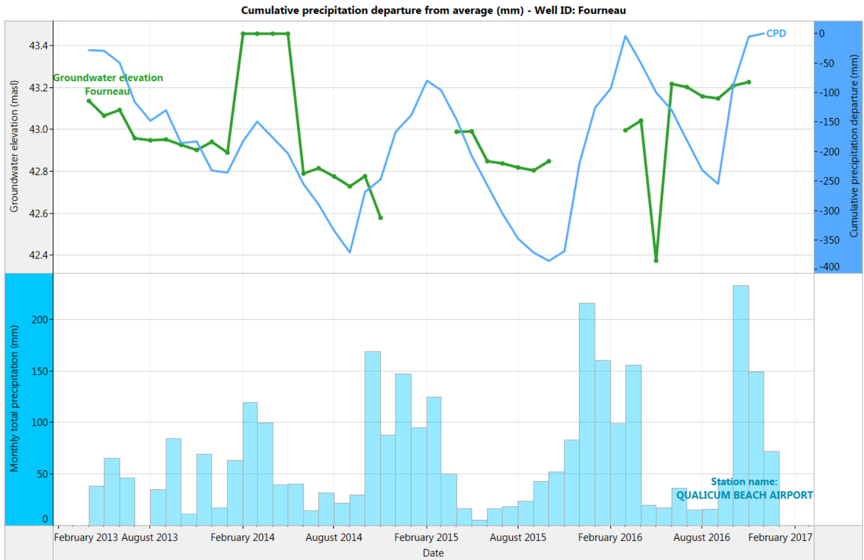
Figure 16. Fourneau: Month end groundwater levels compared to cumulative precipitation departure curve and total monthly precipitation (2013-2016)
