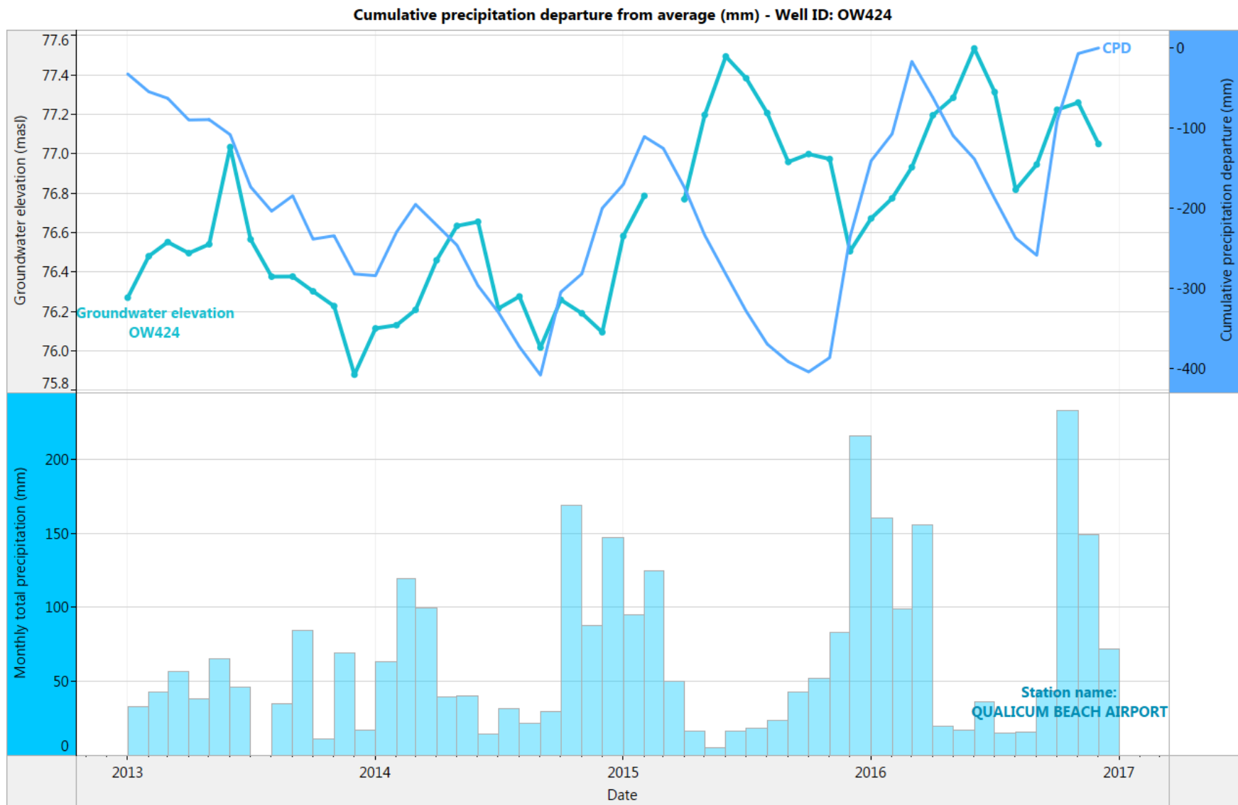
Figure 20. OW424: Month end groundwater levels compared to cumulative precipitation departure curve and total monthly precipitation (2013-2016)
