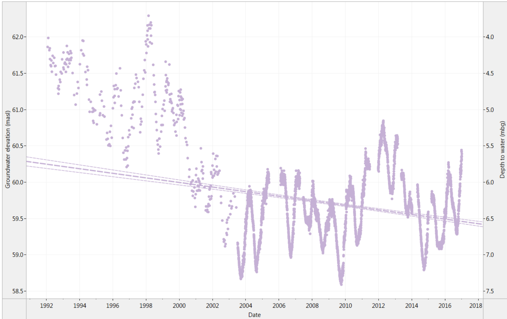
Figure 8. OW314: Historical daily water level (1992-2016) and trend line estimation (1992-2016)
