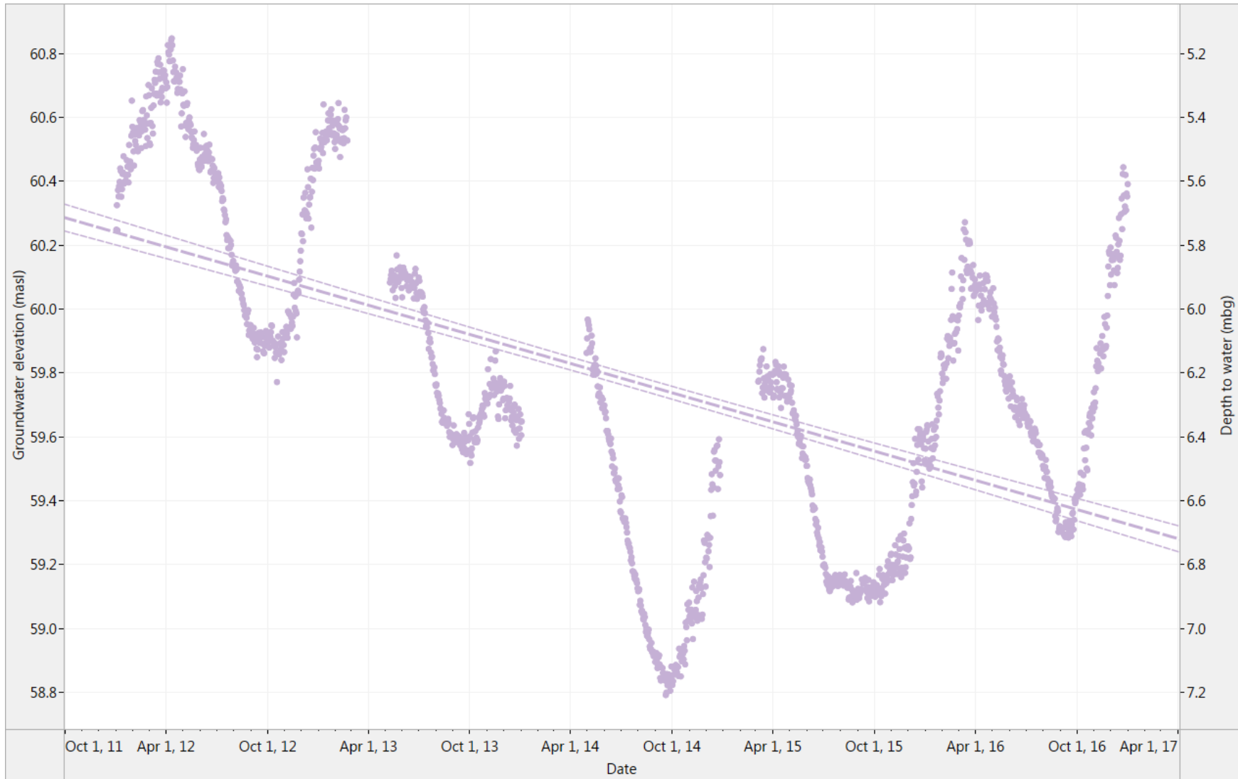
Figure 9. OW314: Water level and trend line estimation for the last five years (2012-2016)
