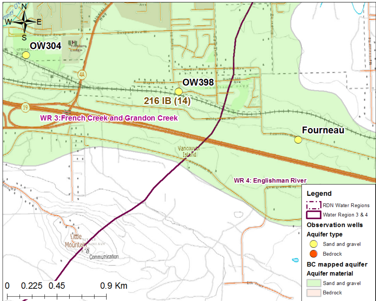
Figure 2. Location of observation wells OW304, OW398 and Fourneau
