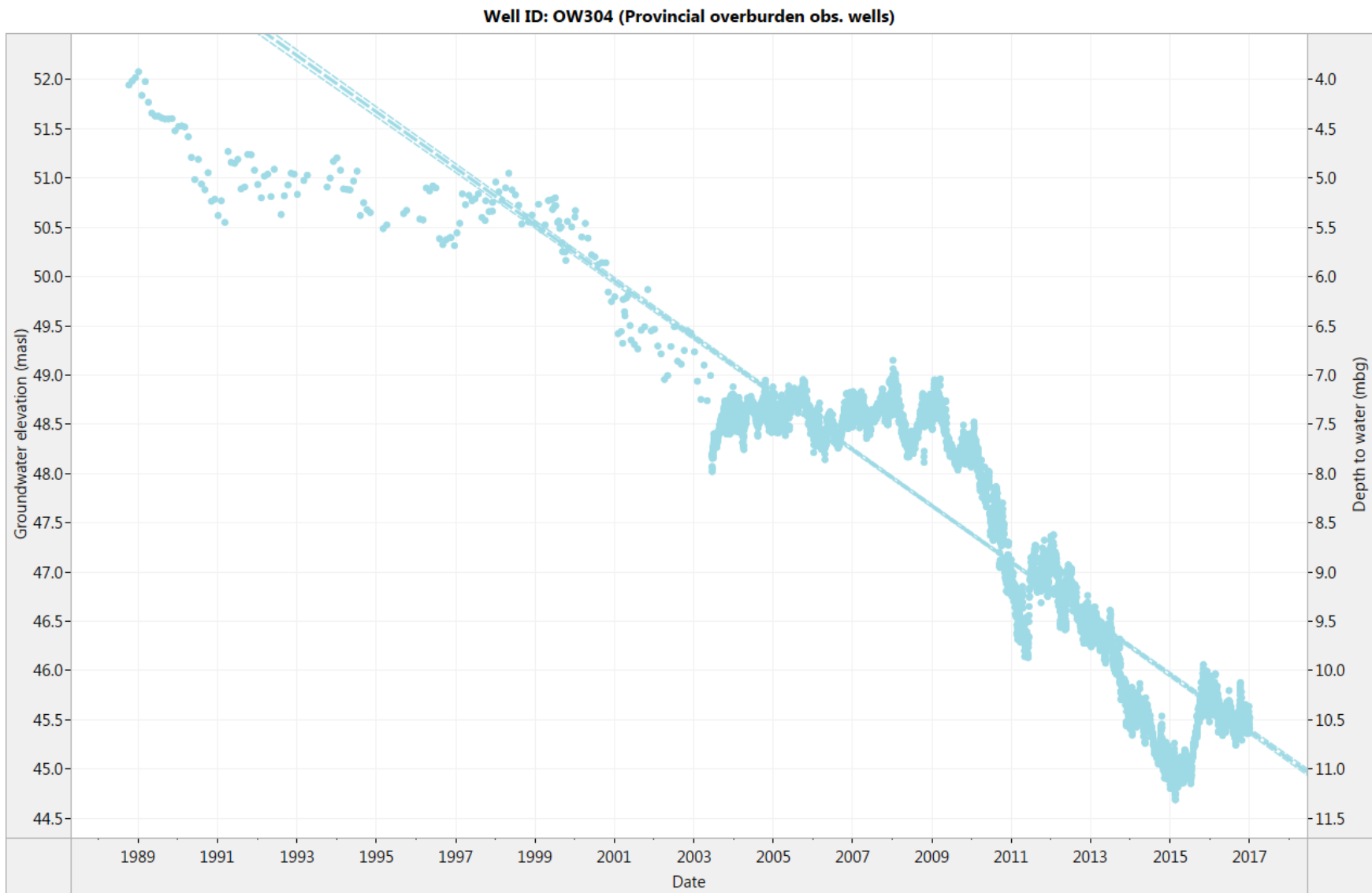
Figure 6. OW304: Historical daily water level (1988-2016) and trend line estimation (1989-2016)
