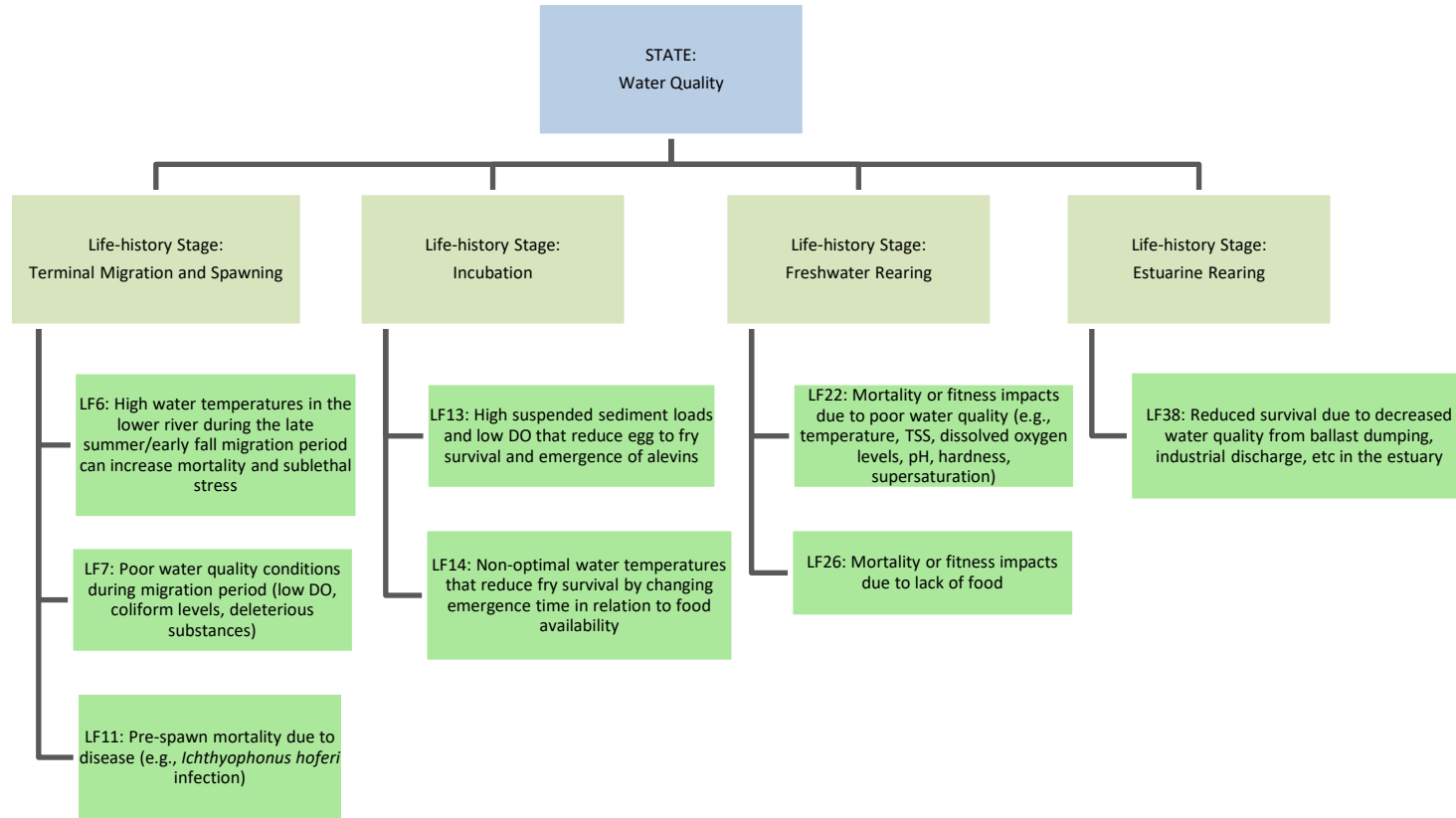
Figure 16. Relationship between water quality, life-history stages, and limiting factors.
