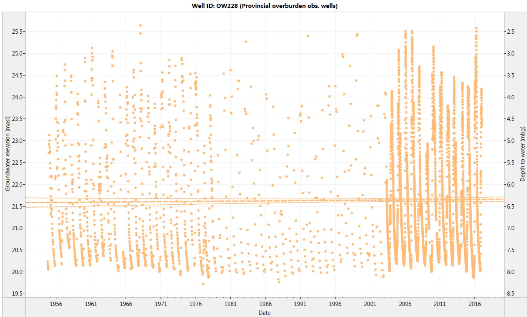
Figure 3. OW 228: Historical daily water level (1954-2016) and trend line estimation (1954-2016)
