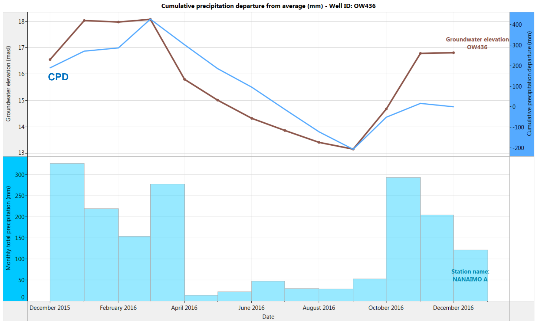
Figure 11. OW436: Month end groundwater levels compared to cumulative precipitation departure curve and total monthly precipitation (2015-2016)
