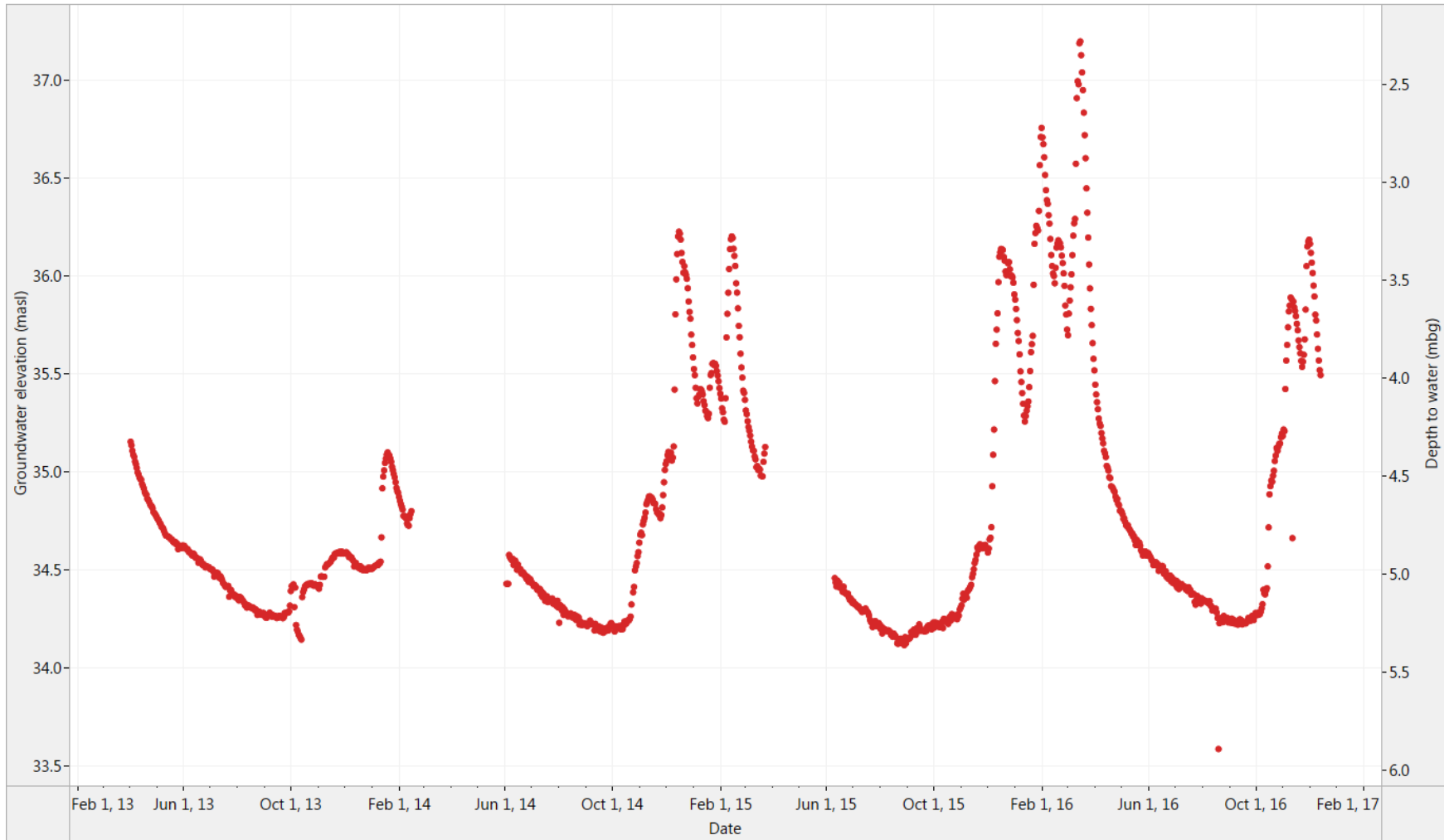
Figure 6. Hallberg: Historical water level (2013-2016)
