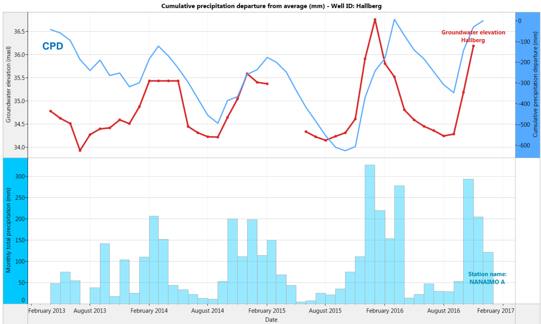
Figure 12. Hallberg: Month end groundwater levels compared to cumulative precipitation departure curve and total monthly precipitation (2013-2016)
