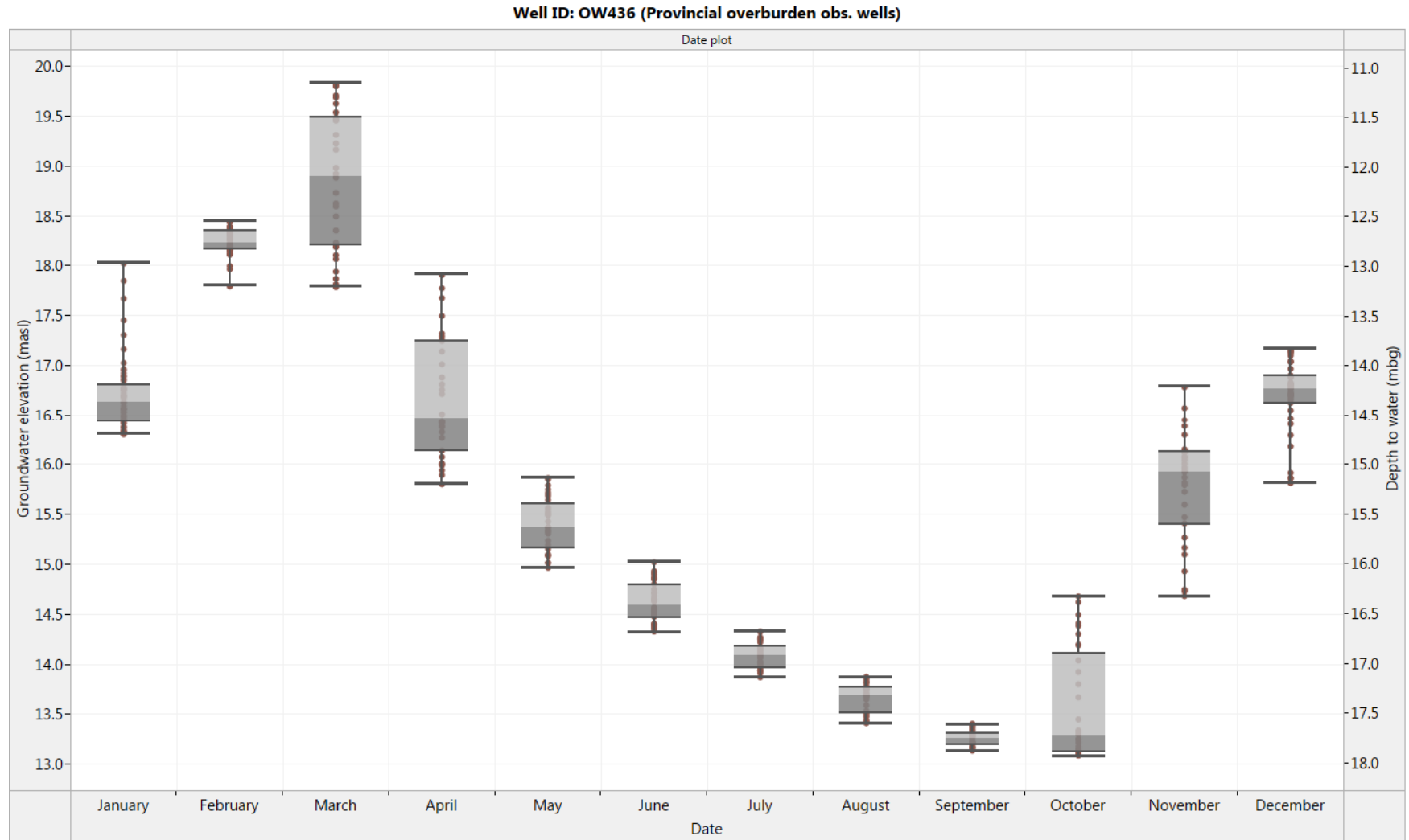
Figure 8. OW436: Box and Whisker diagram for historical monthly groundwater level fluctuation (2015-2016)
