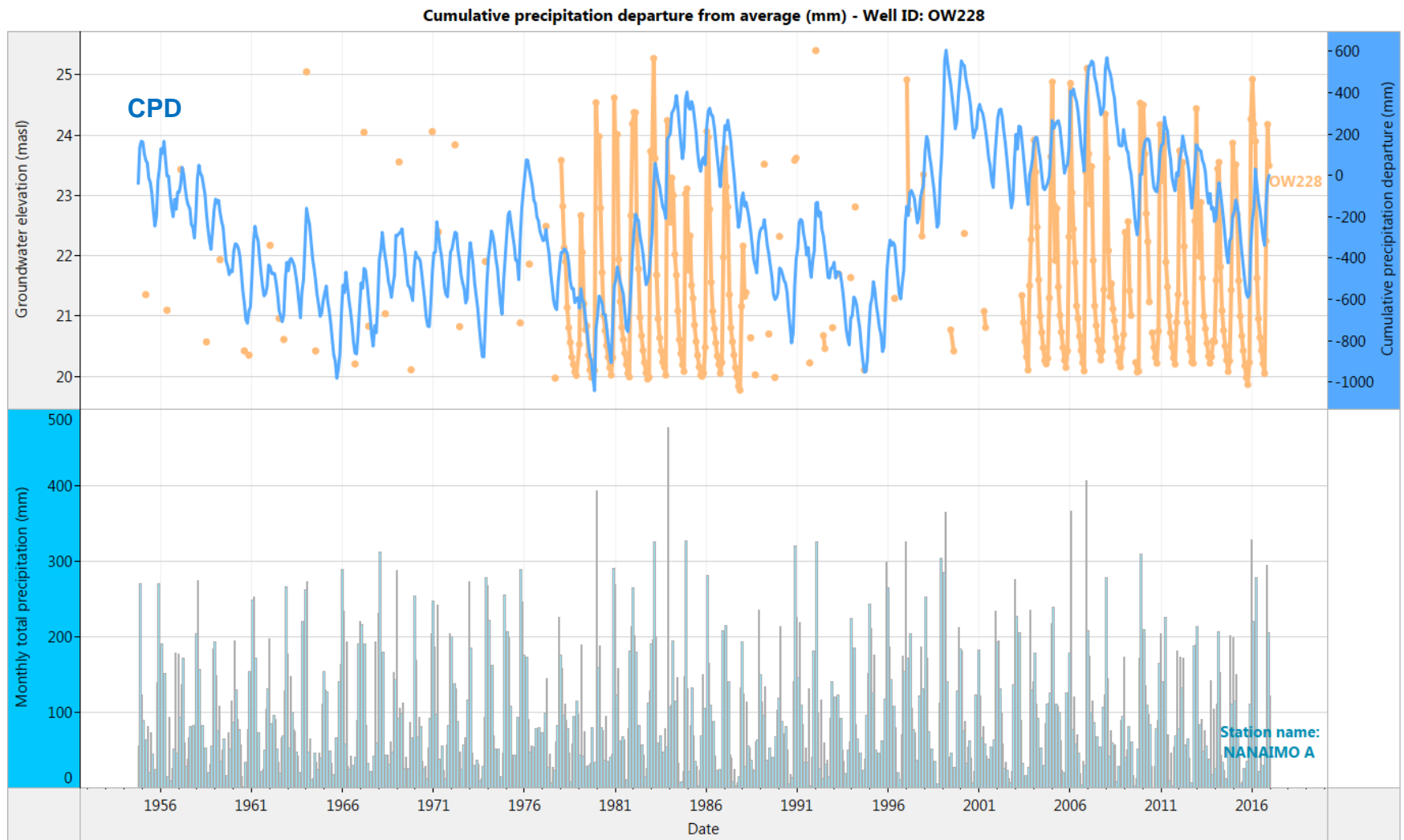
Figure 10. OW228: Month end groundwater levels compared to cumulative precipitation departure curve and total monthly precipitation (1954-2016)
