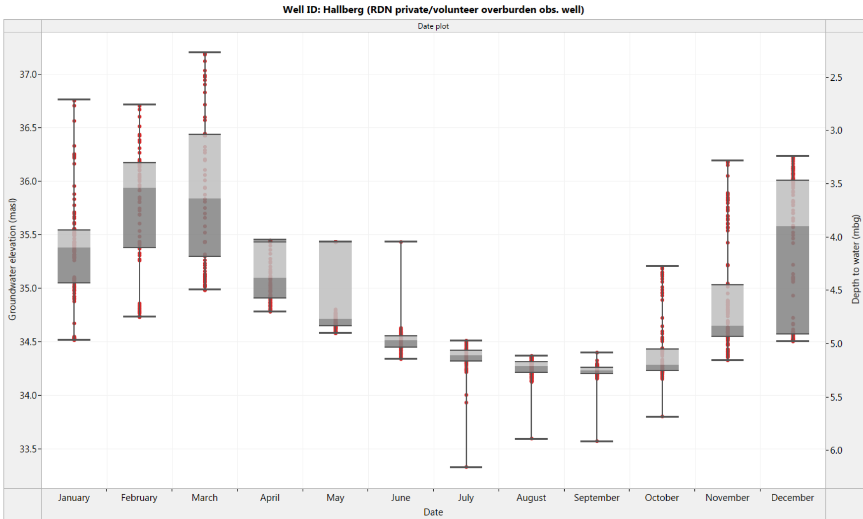
Figure 9. Hallberg: Box and Whisker diagram for historical monthly groundwater level fluctuation (2013-2016)
