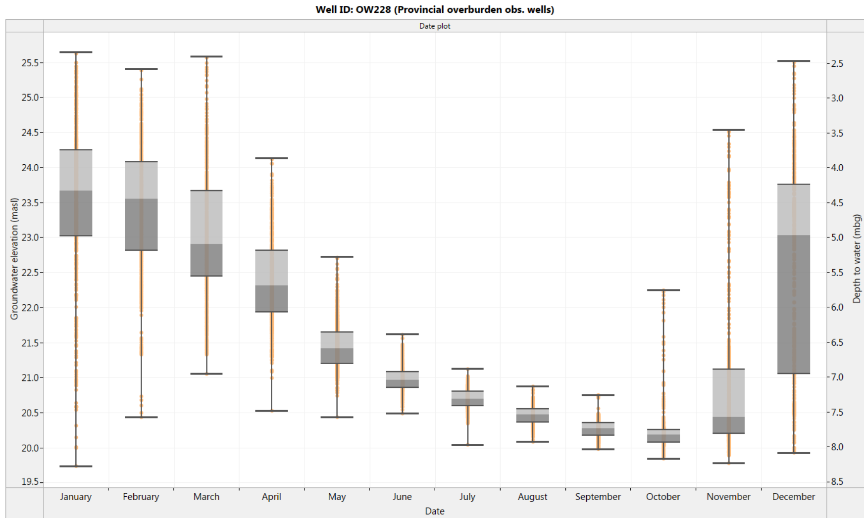
Figure 7. OW228: Box and Whisker diagram for historical monthly groundwater level fluctuation (1991-2016)
