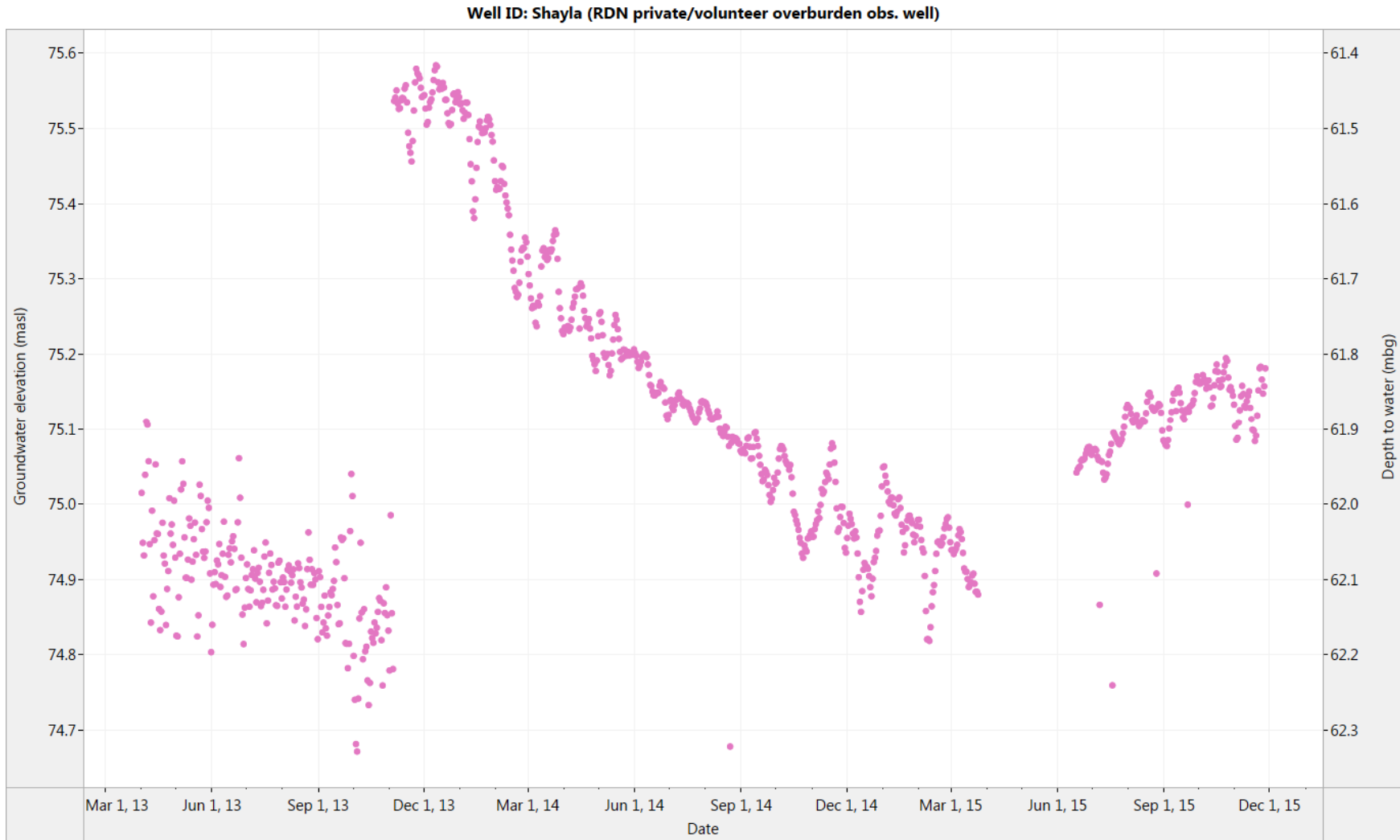
Figure 3. Shayla: Historical water level (2013-2015)
