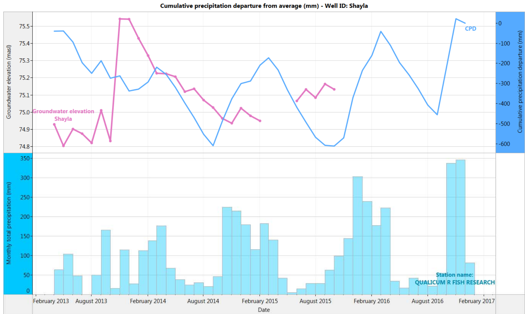
Figure 5. Shayla: Month end groundwater levels compared to cumulative precipitation departure curve and total monthly precipitation (2013-2015)
